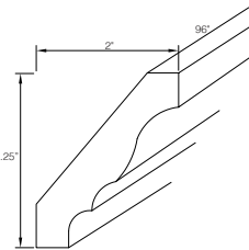
Traditional Crown Molding - TCM8
