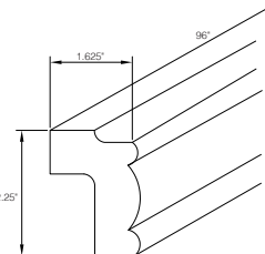
Traditional Light Rail Molding - LR8
