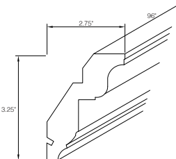
Royal Crown Molding - RCM8
