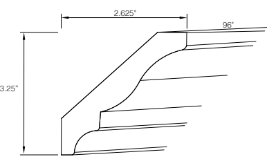
Large Crown Molding - LCM8
