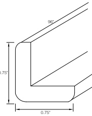
Outside Corner Molding - OC8
